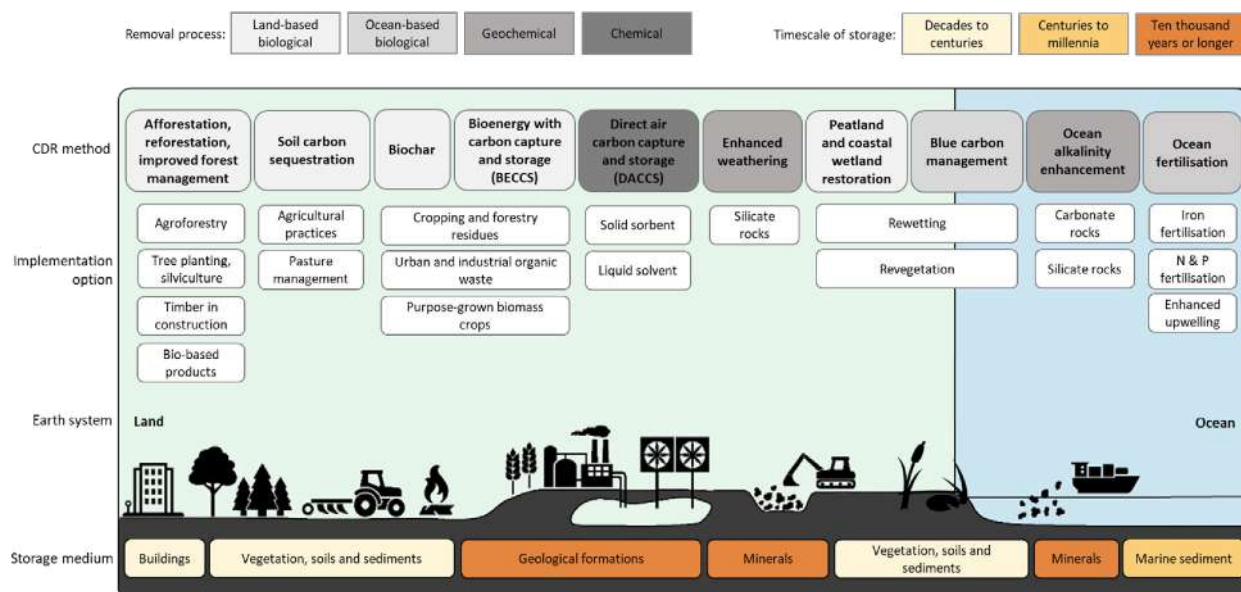
Figure 1: CDR is the physical, permanent, and net removal of greenhouse gases from the atmosphere. Once emitted, CO 2 may remain in the atmosphere for hundreds of years. A variety of options to remove and store atmospheric are available, but ensuring that these activities result in true CDR requires managing storage to prevent or compensate for any potential re-emissions, and to ensure that the quantification of CDR accounts for the greenhouse gas emissions in the removal and storage processes and their supply chains.
